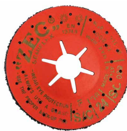
ABRASIVE HOOF DISC "ZEC - SEMIFLEX" SILICON CARBIDE (GRAIN 16) Ø 115 MM - 4,5"
