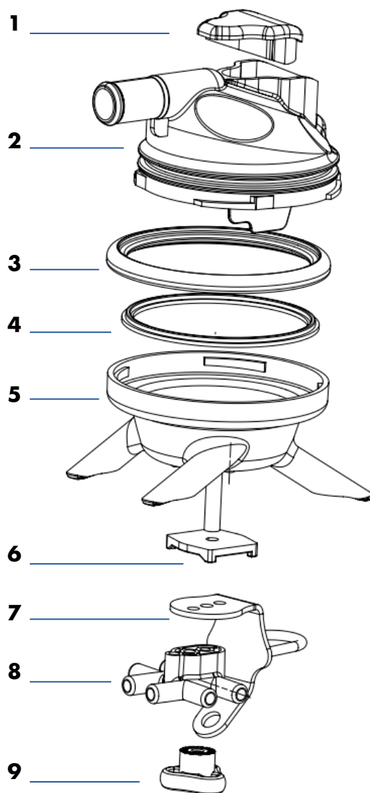
MILKING CLAW IN POLYSULFONE "VISTAR 450" 370 CC WITHOUT VALVE
