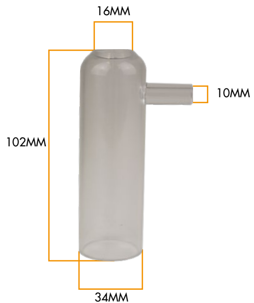
PLASTIC MILKING LINER CASE FOR SHEEP MILKING LINER 04.04.0402
