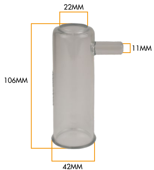
PLASTIC MILKING LINER CASE OR SHEEP MILKING LINER 04.04.0406
