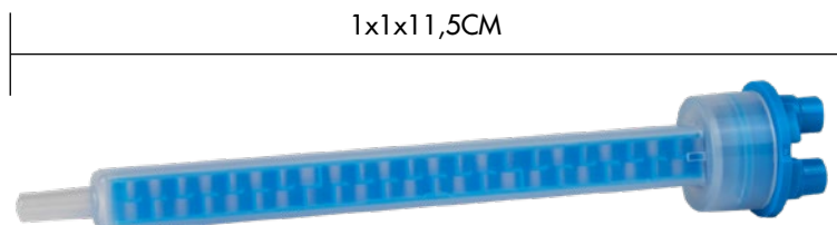
MIXING TIP BLUE WITH SYMMETRICAL FIT FOR TWO-COMPONENT HOOF GLUE 200 ML TUBE - F-SYSTEM FITTING (10)
