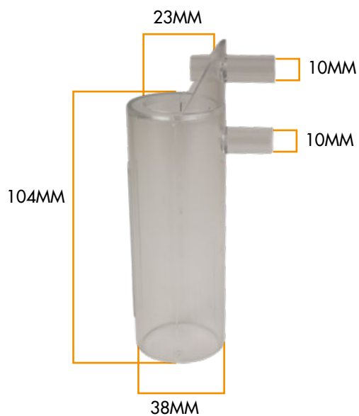
PLASTIC MILK LINER CASE FOR SHEEP MILKING LINER 04.04.0404
